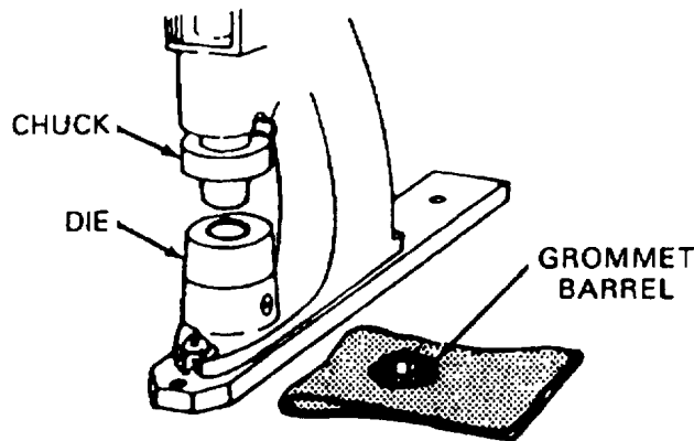
GROMMET BARREL INSERTED IN MATERIAL HOLE
