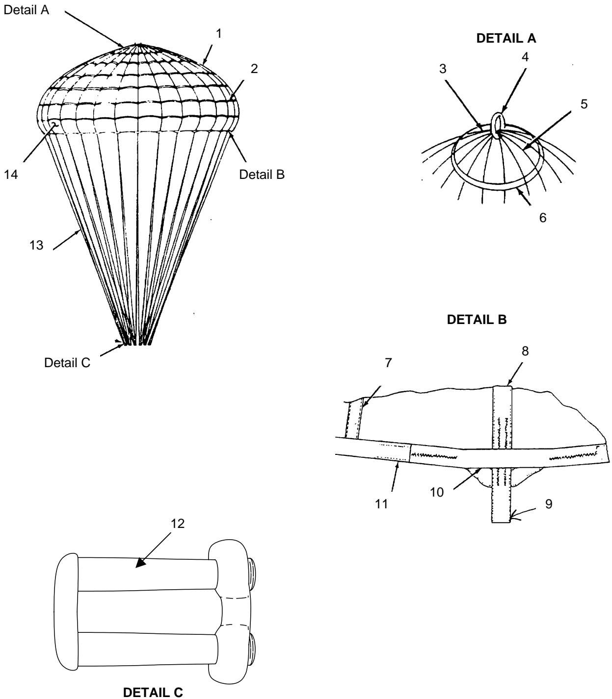
Figure 1. Canopy, 28-Foot Diameter
